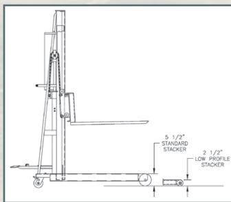
Low Profile Stacker Outtrigger Option - 2.5" Outtrigger Height
